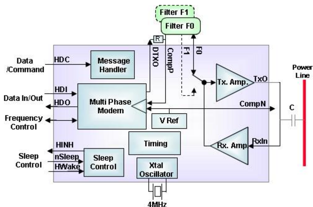
Figure 2.1 - SIG60 logical blocks
