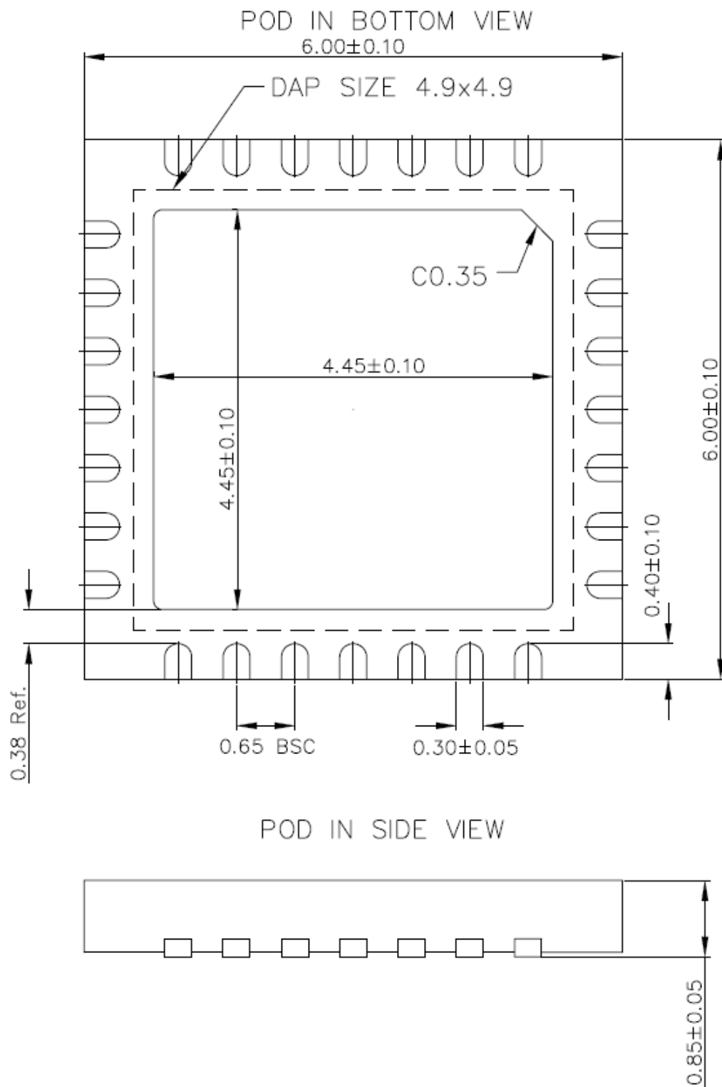
Figure 5.1 – QFN28 mechanical dimensions
